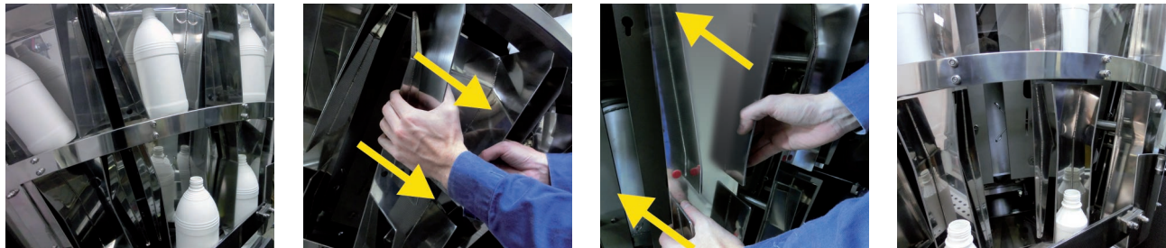
Replacement of the funnel
